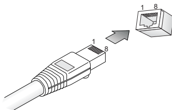
Figure B-1 RJ-45 Connector Pin Numbers
