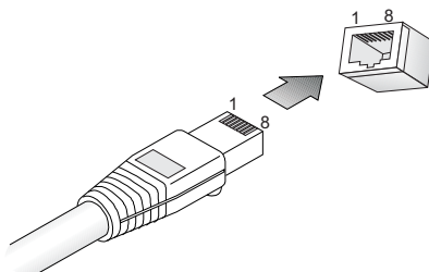
Figure 3-9 Serial Port (RJ-45) Pin-Out
