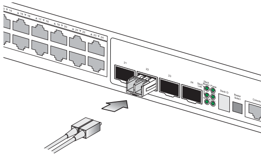
Figure 4-3 Making Connections to SFP Transceivers
