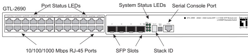
Figure 1-1 Front Panel
