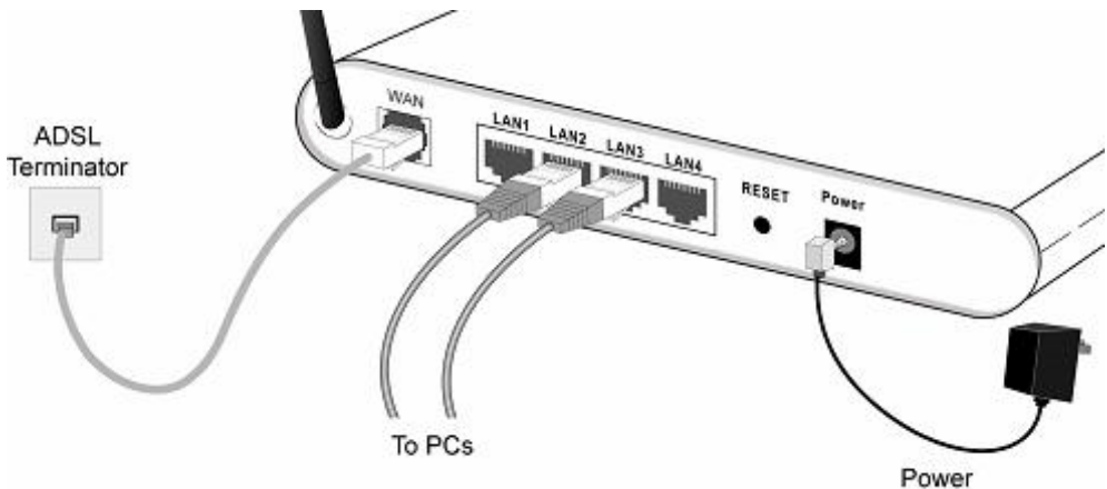
Figure 4: Installation Diagram
