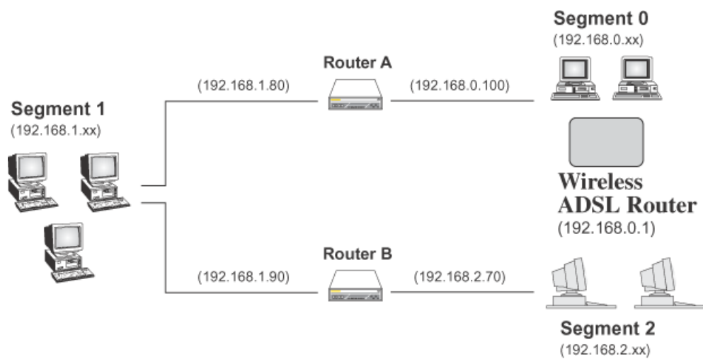
Figure 63: Routing Example
