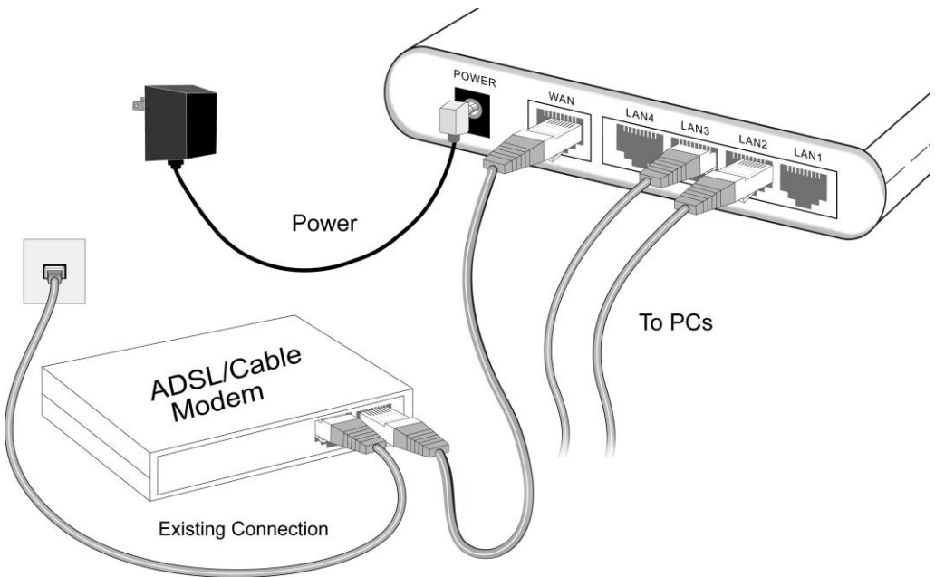
Installation Diagram
