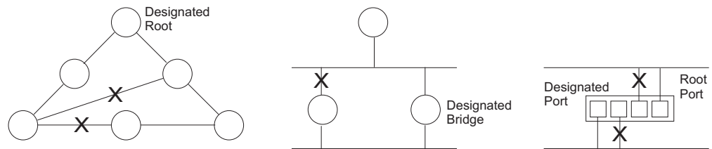
Figure 44: STP Root Ports and Designated Ports
