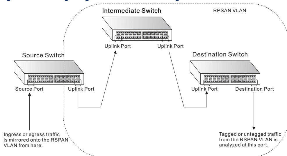
Figure 90: Configuring Remote Port Mirroring
