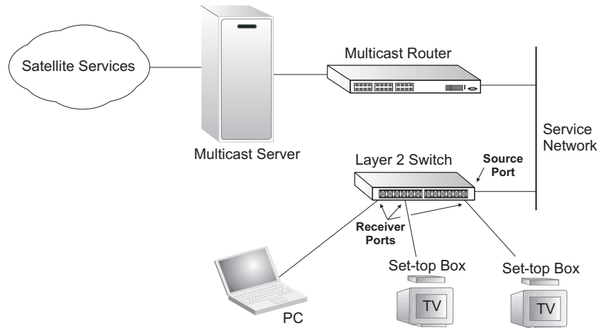
Figure 52: MVR Concept
