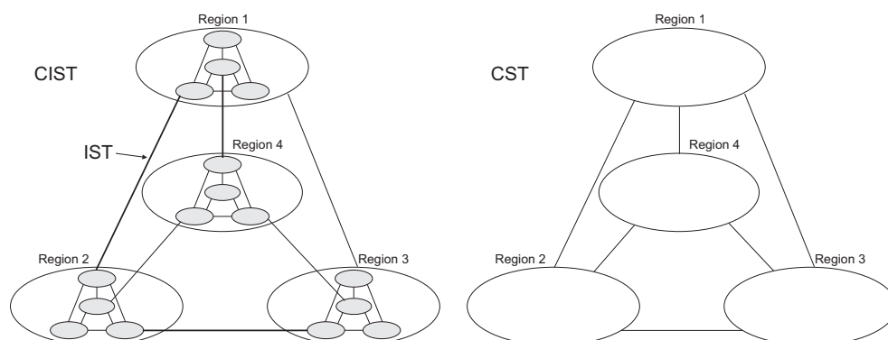
Figure 46: Common Internal Spanning Tree, Common Spanning Tree, Internal Spanning Tree
