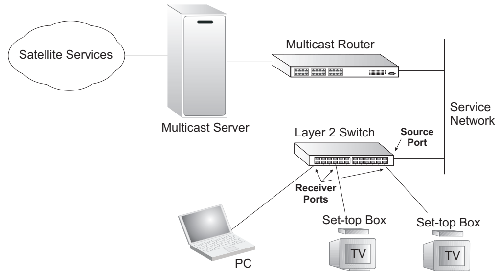
Figure 53: MVR Concept
