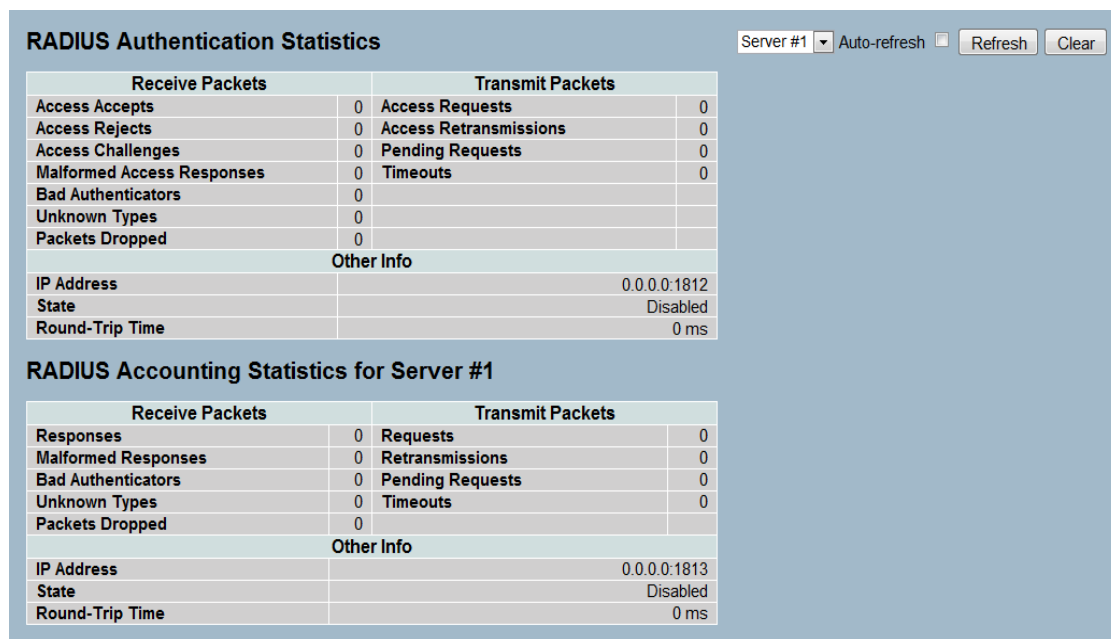
Figure 4-6.3: The RADIUS Authentication Statistics Server
