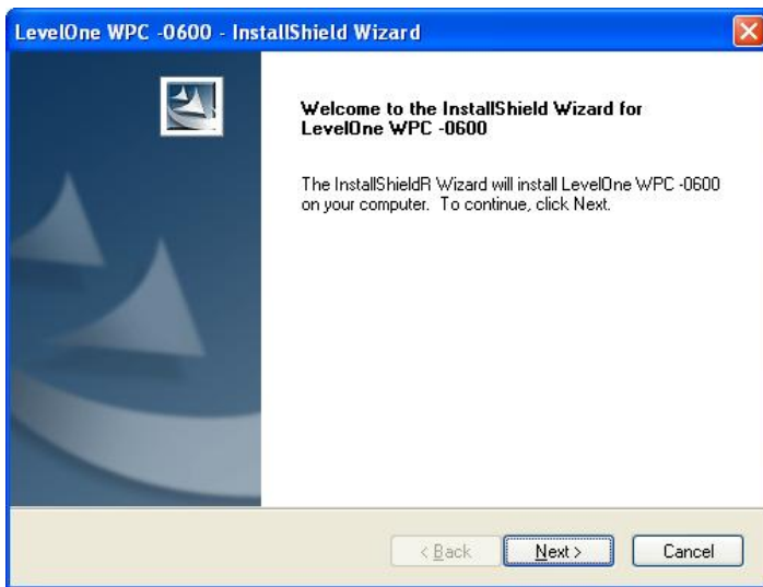
Figure 1: Start Installation
