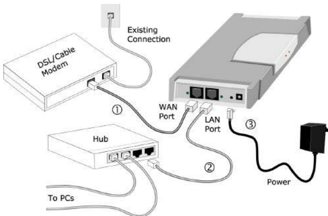
Figure 6: Installation Diagram
