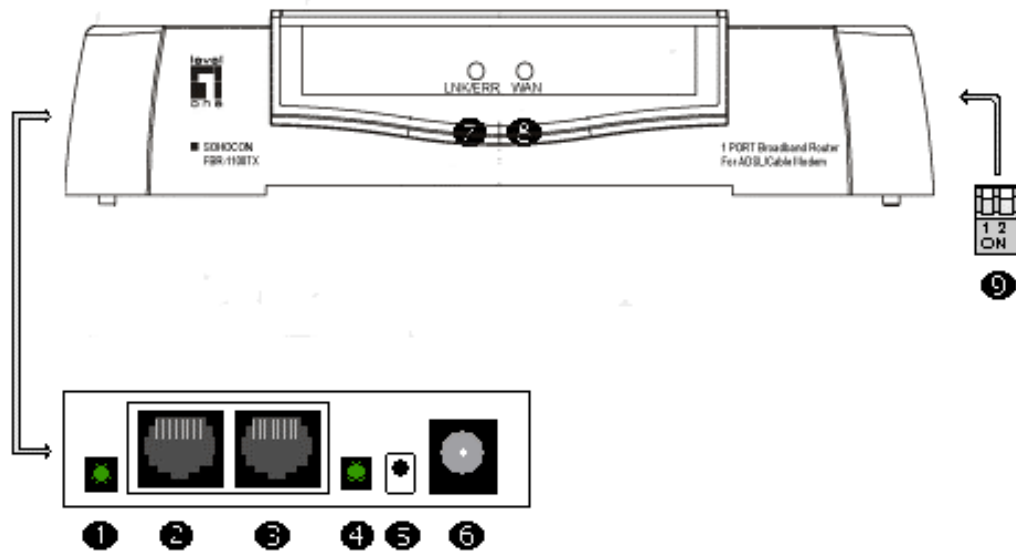
Figure 2: Components - FBR-1100TX
