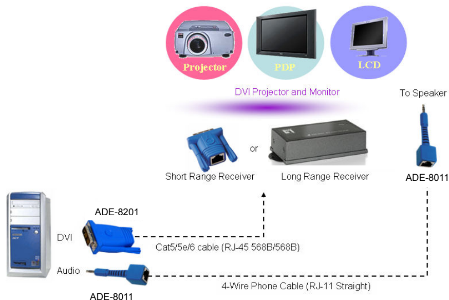
Extended Connection of DVI-D with Audio
