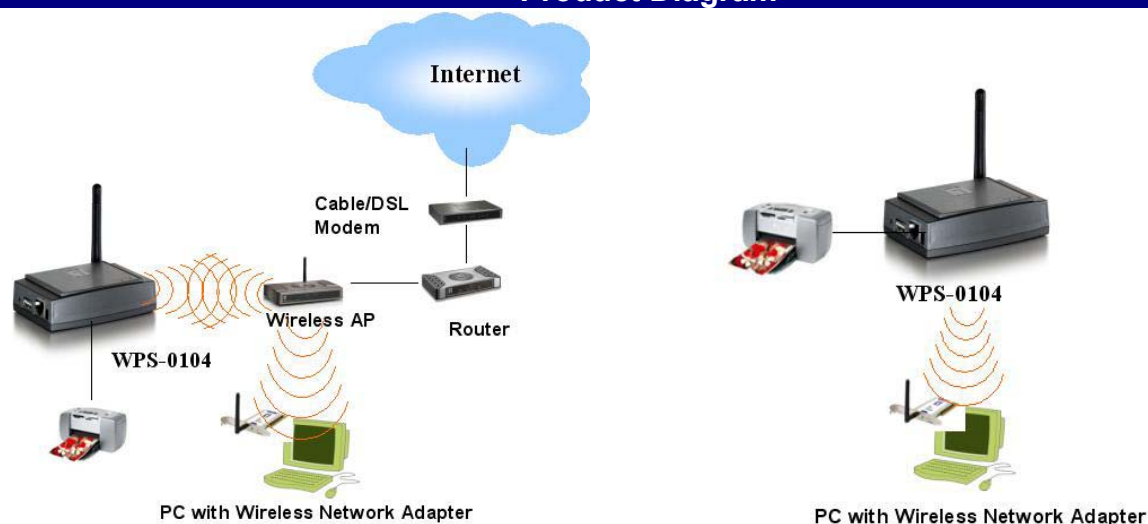
WCS-0104 Diagram (Infrastructure mode)
